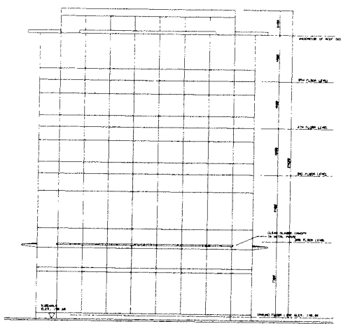
WEST ELEVATION
