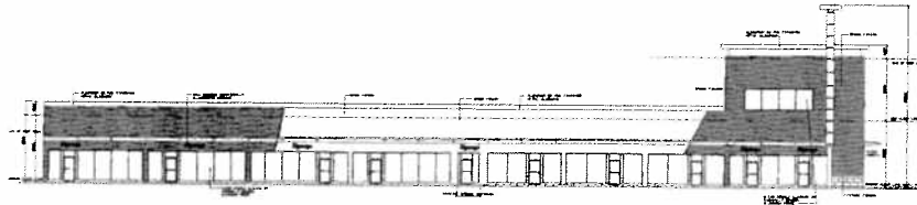
BUILDING 1 – SOUTH ELEVATION (PARKING)
