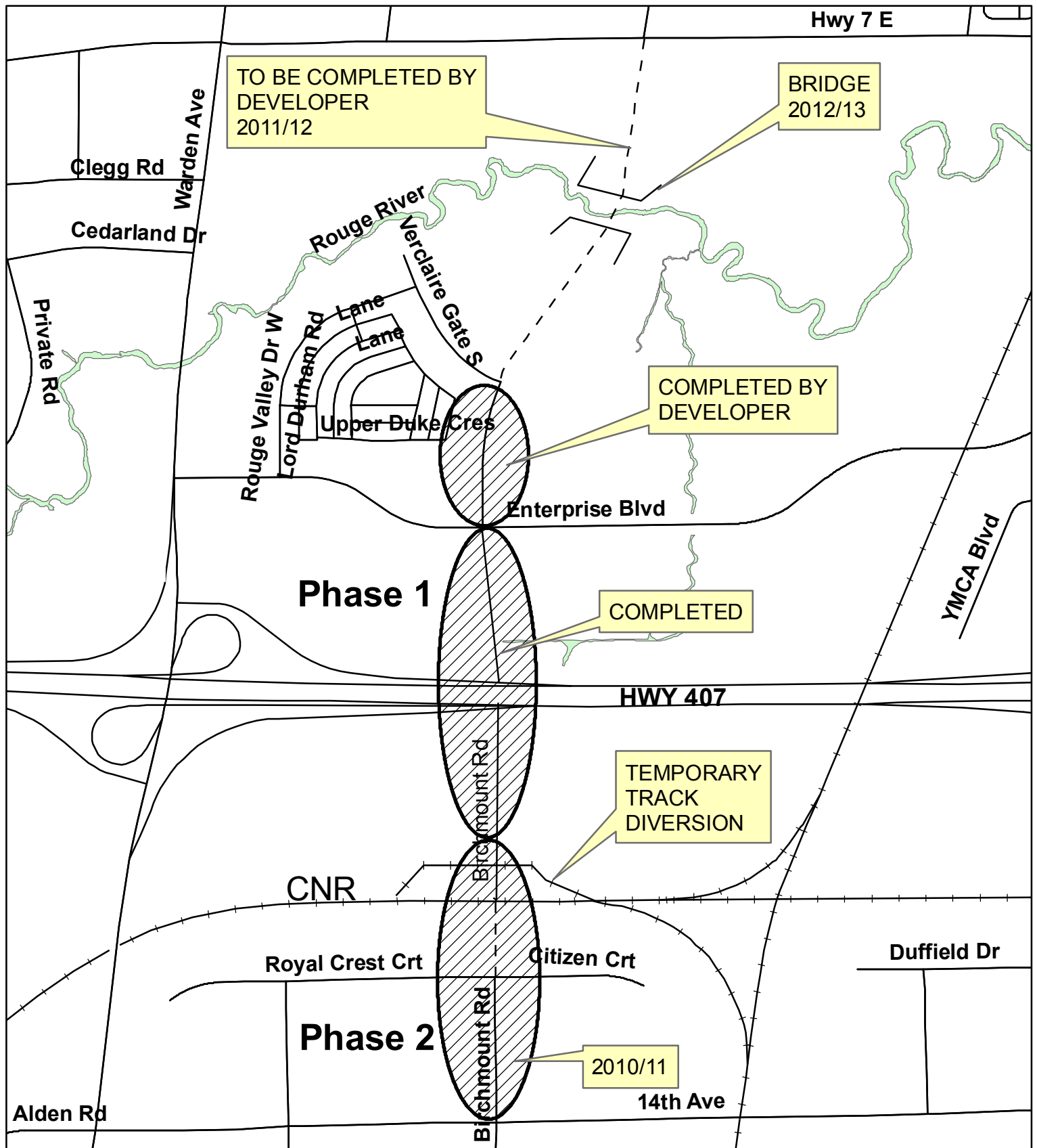
Figure 1 Birchmount Road Phase 1 and 2
