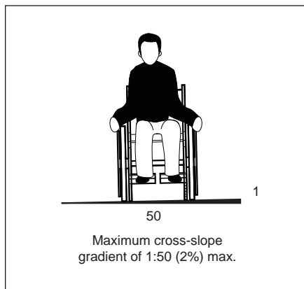
Figure 49: Cross-Slope
