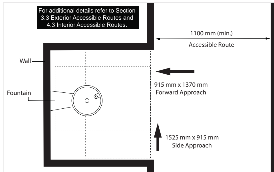
Figure 18: Clear Floor Space Requirements and Approach at Drinking Fountain - Plan View
