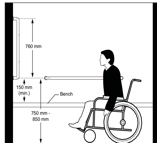
Figure 92b: Grab Bar Dimensions
