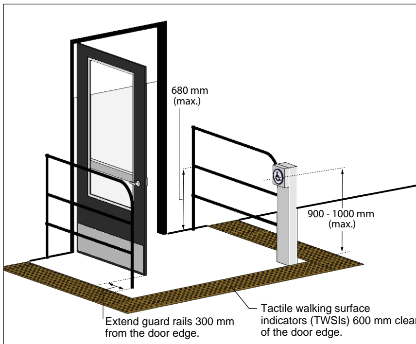
Figure 42: Doors on Accessible Routes
