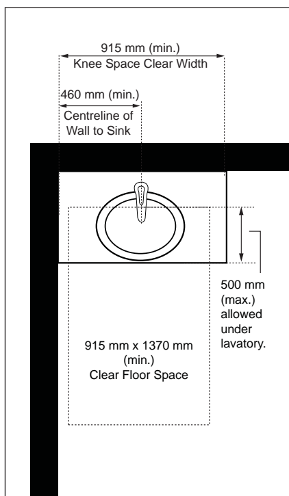
Figure 57a: Lavatories - Plan View
