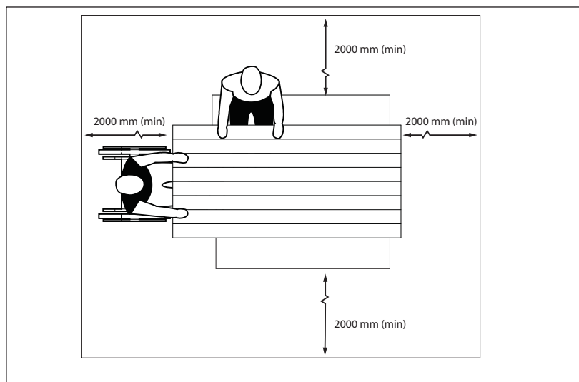
Figure 97a: Picnic Table Design and Features - Plan View
