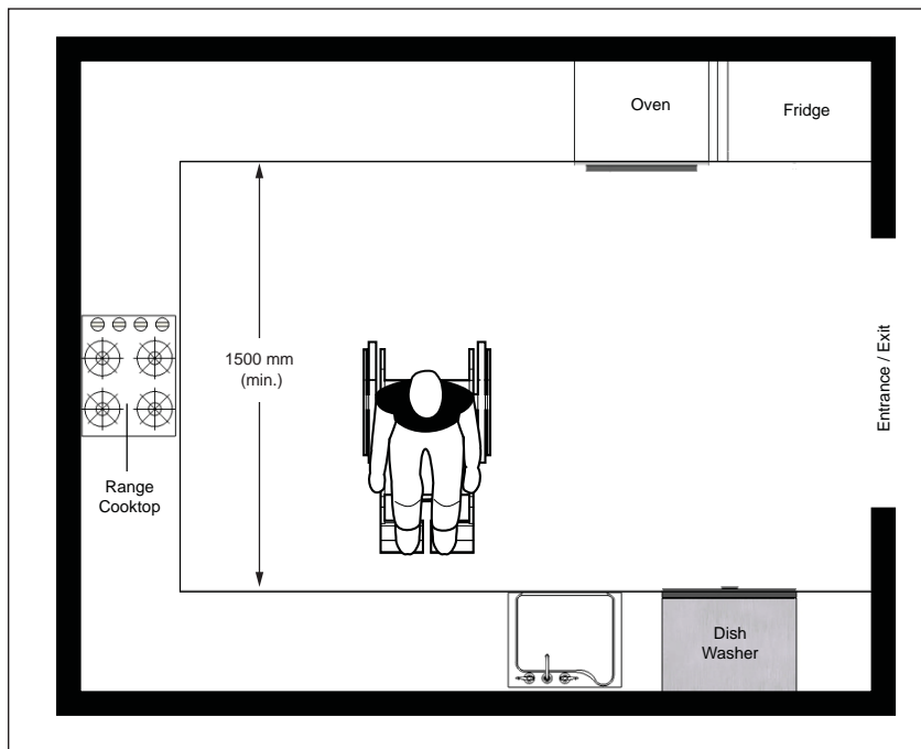
Figure 82: U-Shaped Kitchen - Plan View
