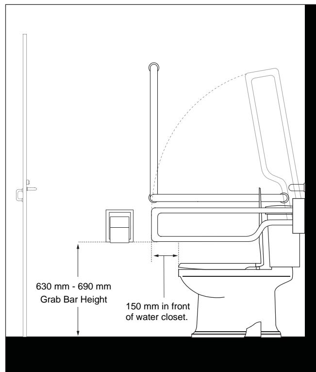
Figure 56b: Fold Down Grab Bars - Elevation View
