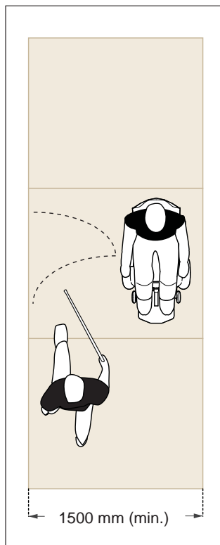
Figure 29a: Minimum Clear Width of Exterior Accessible Route
