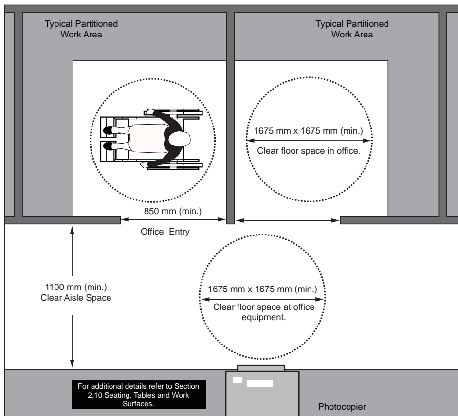
Figure 88: Common-Use Work Areas - Plan View
