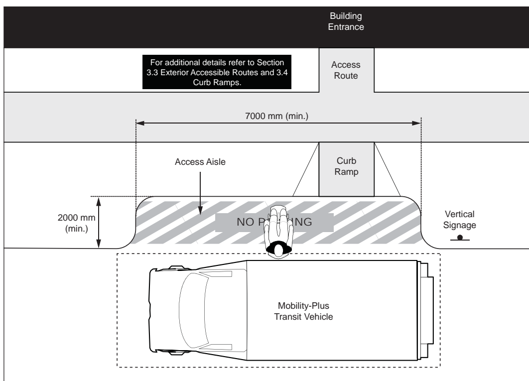
Figure 27: Passenger Loading Zone - Plan View
