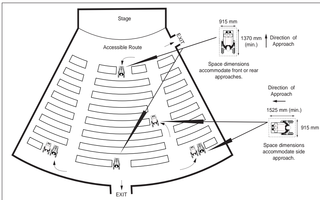
Figure 77: Accessible Seating Plan - Example of Viewing Positions
