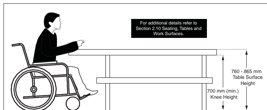
Figure 97b: Picnic Table Design and Features - Elevation View
