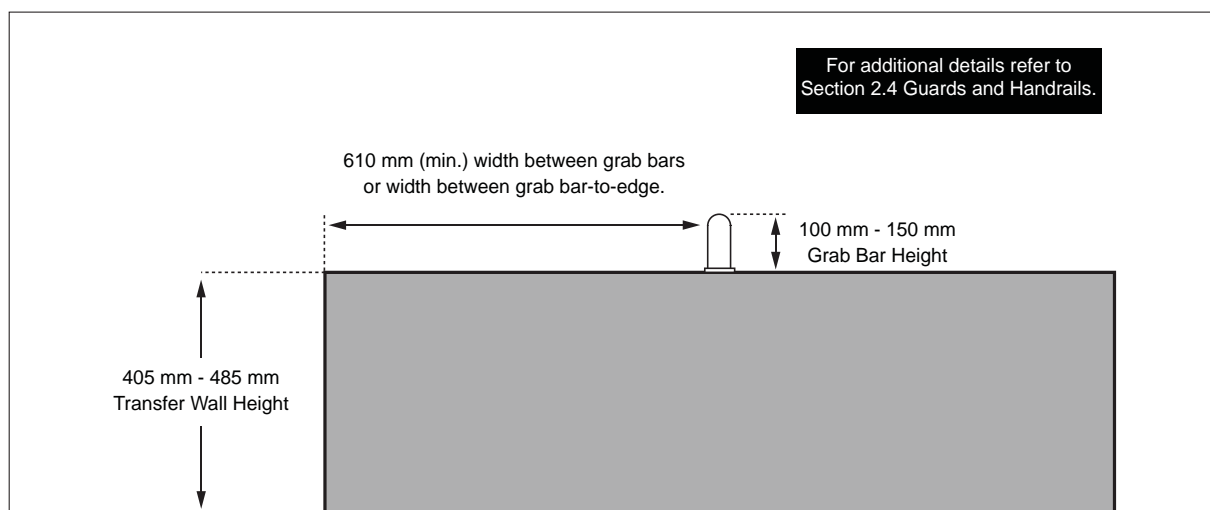
Figure 91: Transfer Wall - Elevation View
