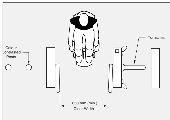
Figure 38: Accessible Controlled Gate
