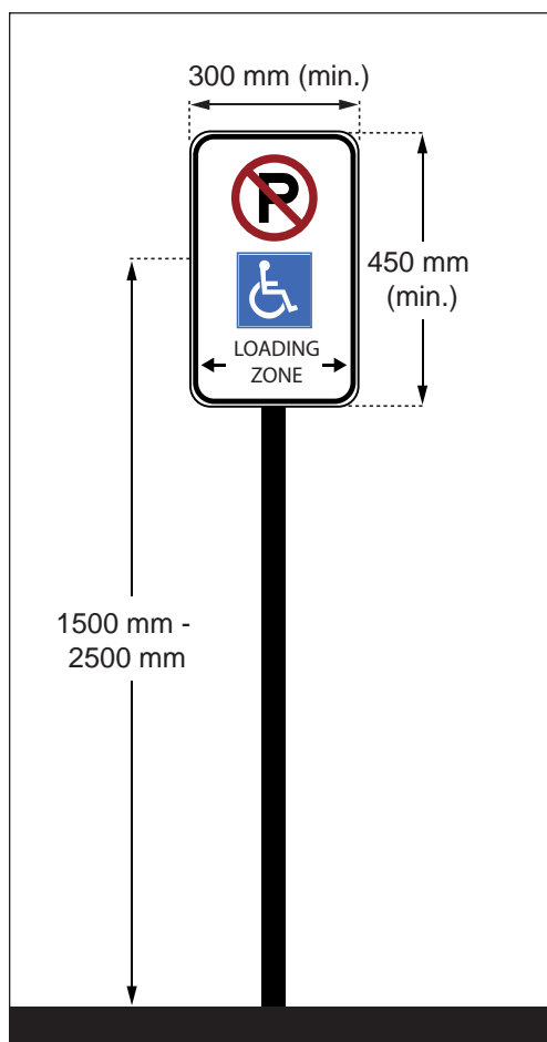
Figure 28: Passenger Loading Zone Vertical Signage
