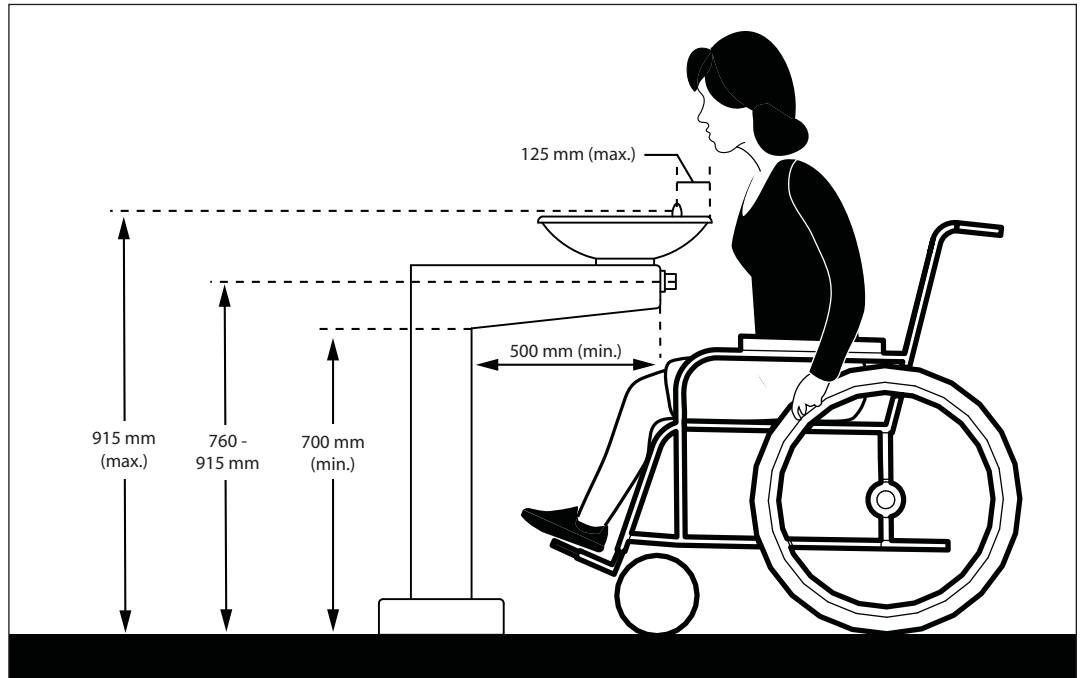
Figure 19: Fountain Design and Layout - Elevation View
