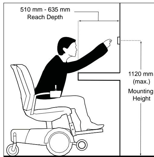
Figure 65b: Obstructed Forward Approach and Reach: Depth 510 to 635 mm (Maximum)
