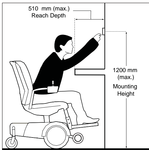
Figure 65a: Obstructed Forward Approach and Reach: Depth 510 mm (Maximum)
