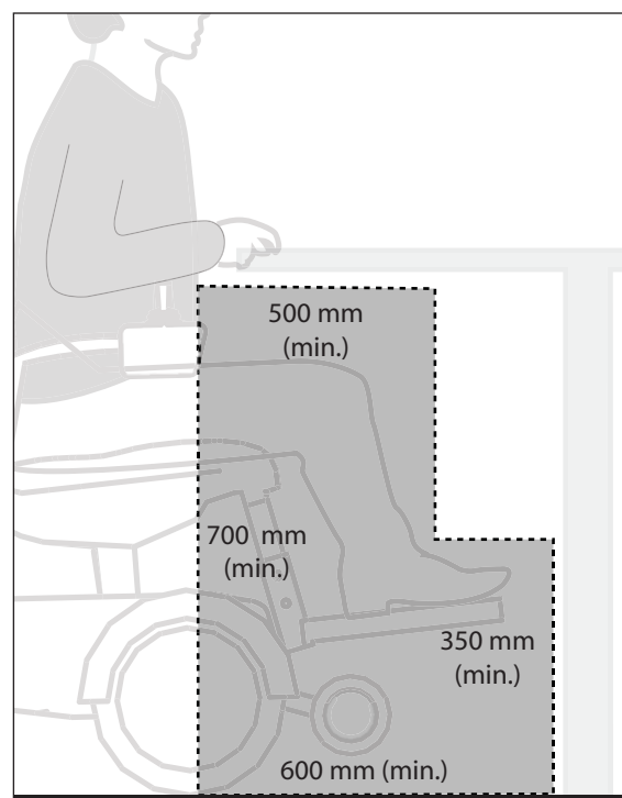
Figure 23b: Knee and Toe Space Dimensions
