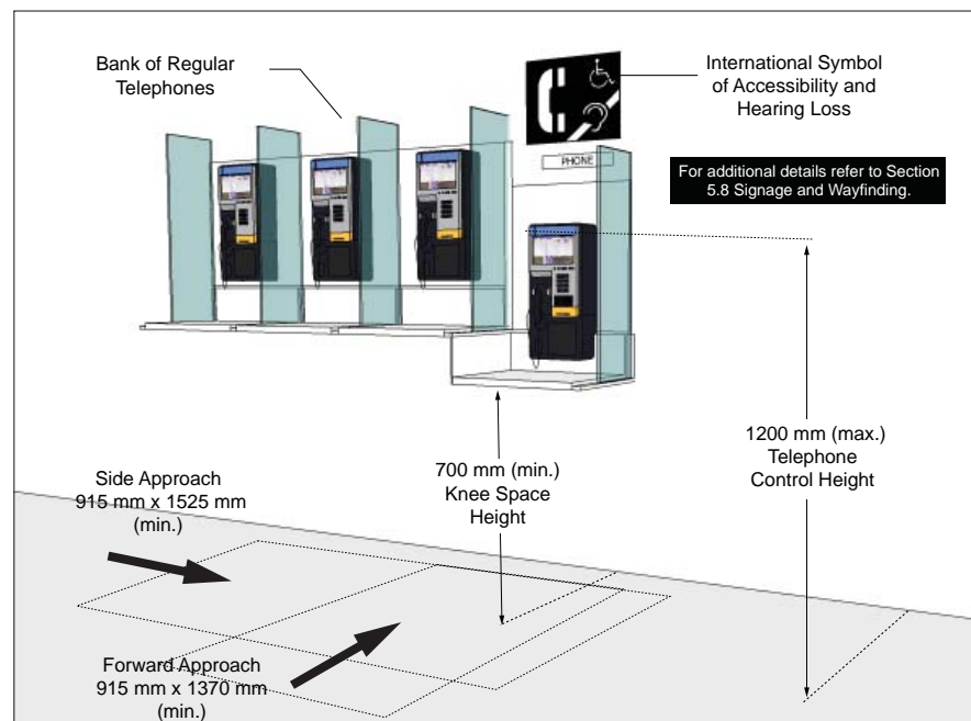
Figure 20: Public Telephone Provisions and Layout
