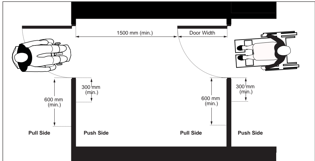
Figure 43: Doors in Series - Plan View
