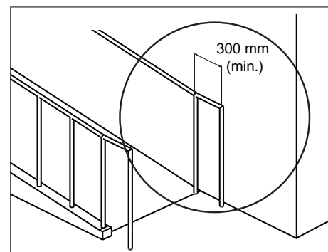
Figure 7c: Handrail Returns to Floor
