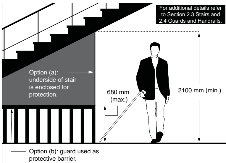
Figure 14: Protection Options Underneath Stairs
