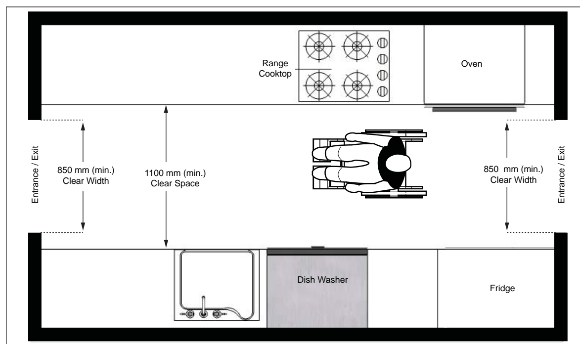
Figure 81: Pass-Through or Galley Kitchen - Plan View
