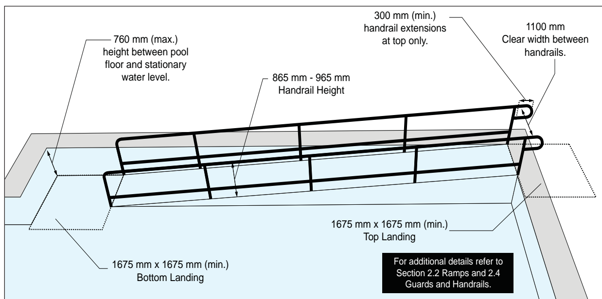
Figure 89: Sloped Entry or Ramp to Swimming Pool
