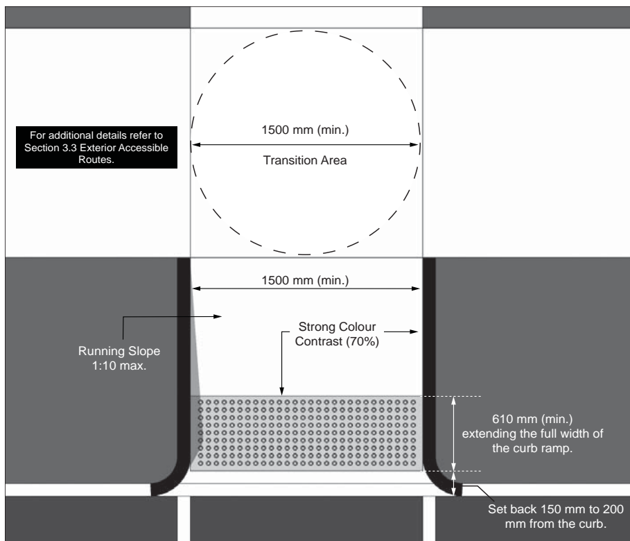
Figure 32: Typical Curb Ramp Design - Plan View
