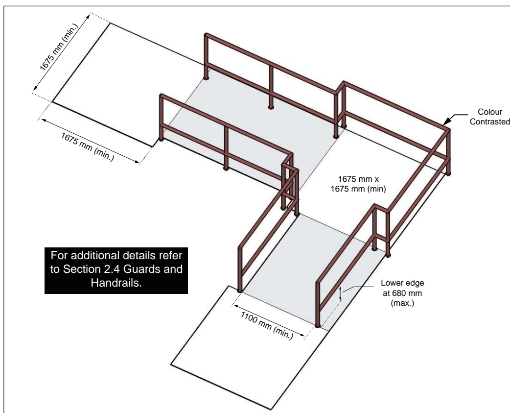
Figure 95: Waiting, Line-up and Queuing Areas
