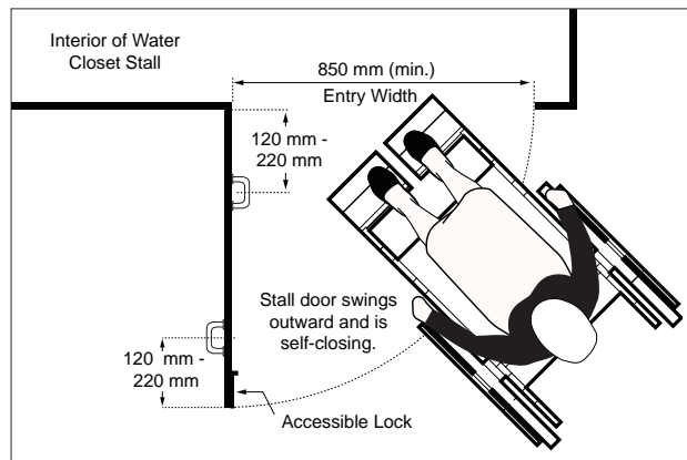
Figure 52: Water Closet Stalls Door Features
