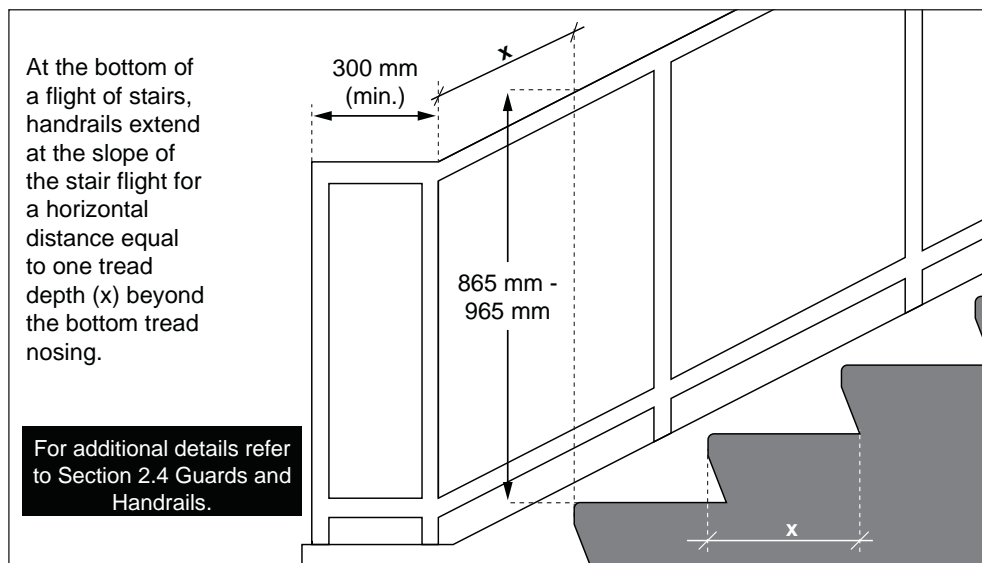
Figure 12: Handrail Extensions at Stairs - Section View
