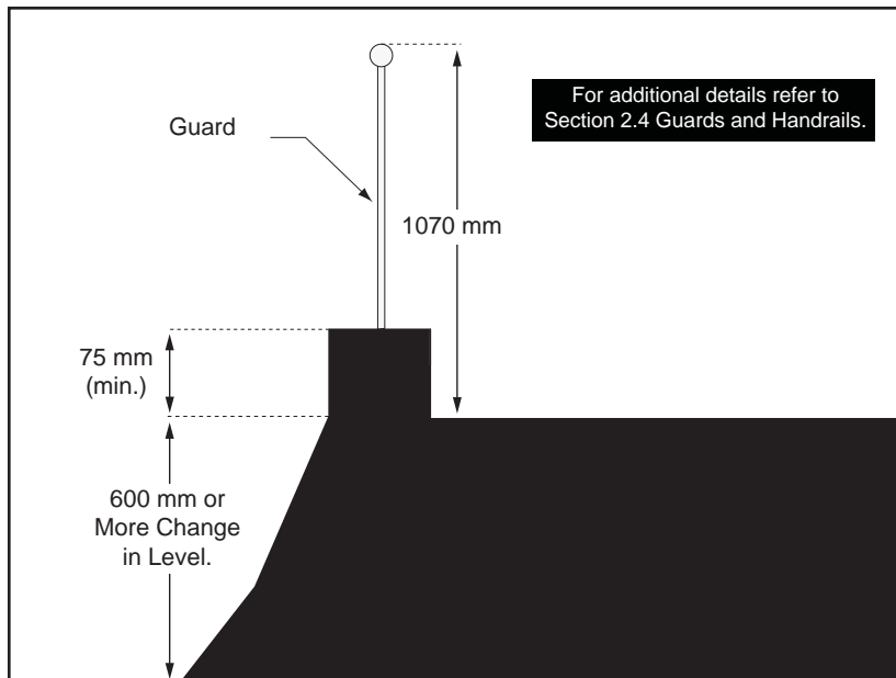
Figure 9: Guard Where Level Change is More than 600 mm Adjacent to Ramp Surface - Section View
