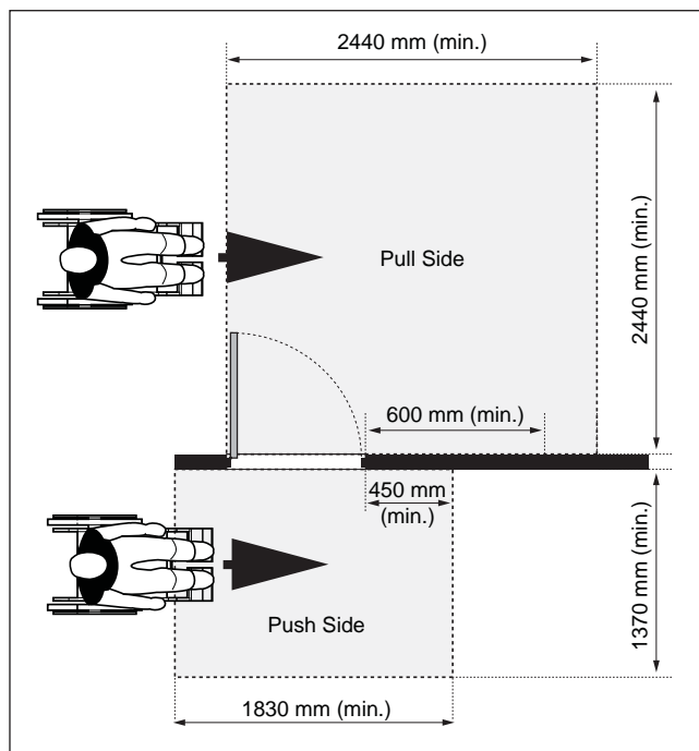
Figure 41c: Hinge Side Approach at Side-Hinged Door - Plan View
