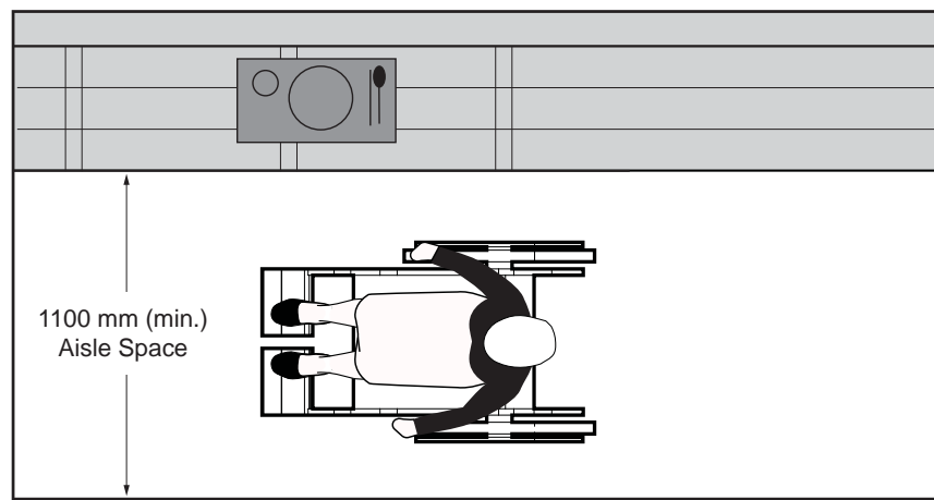
Figure 80b: Aisle Width - Plan View
