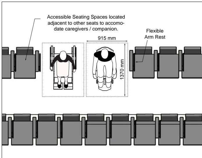
Figure 76: Accessible Seating Space Dimensions
