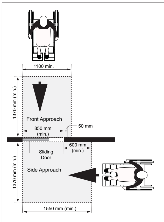
Figure 41b: Front and Side Approach at Sliding Door - Plan View
