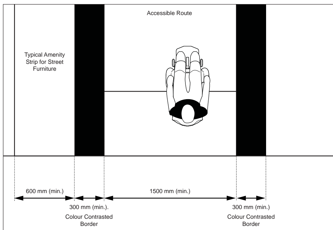
Figure 34: Typical Amenity Strip for Street Furniture Placement
