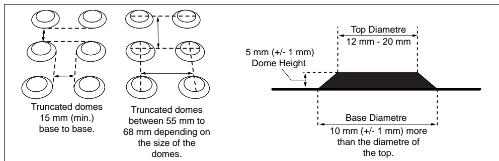
Figure 17: Truncated Dome Specification
