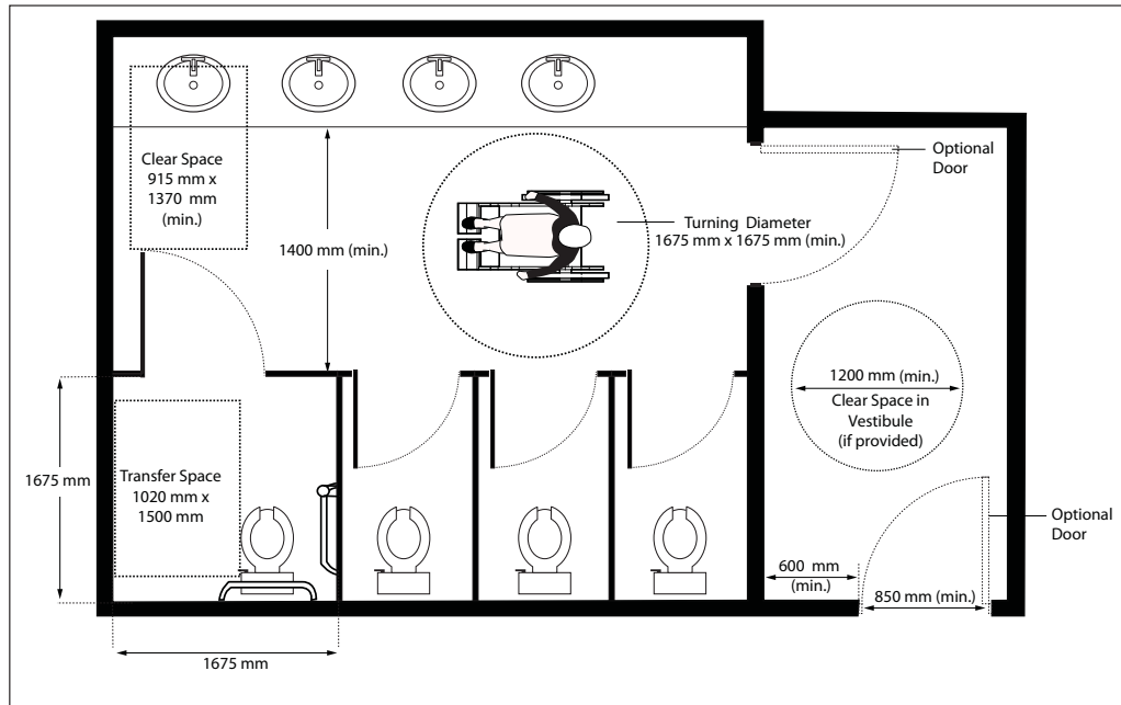
Figure 50: Example of Multiple Occupancy Washroom Layout
