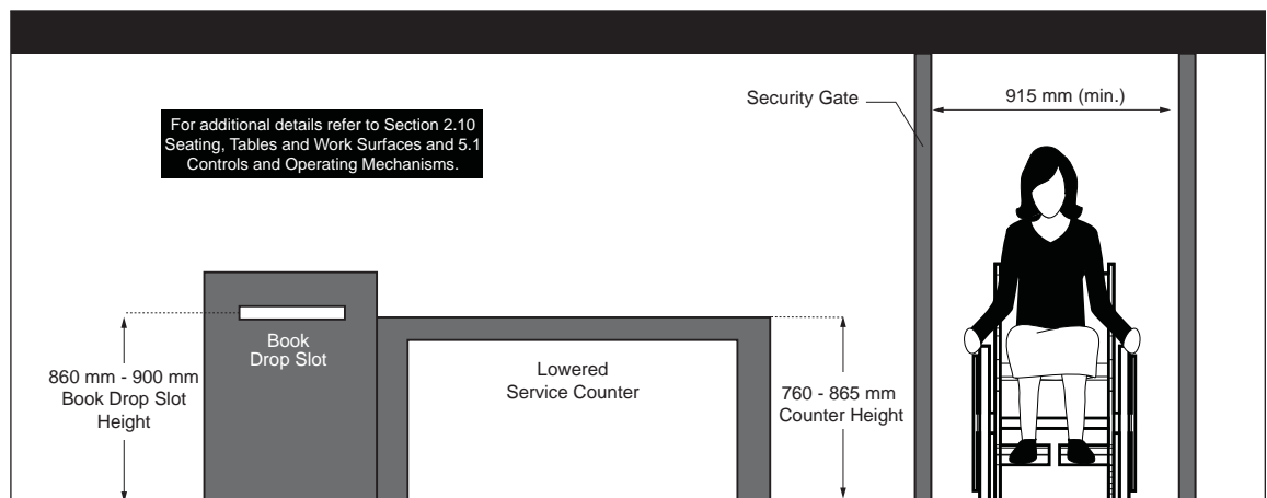
Figure 86: Library Security Gate, Service Counter and Book Drop Slot
