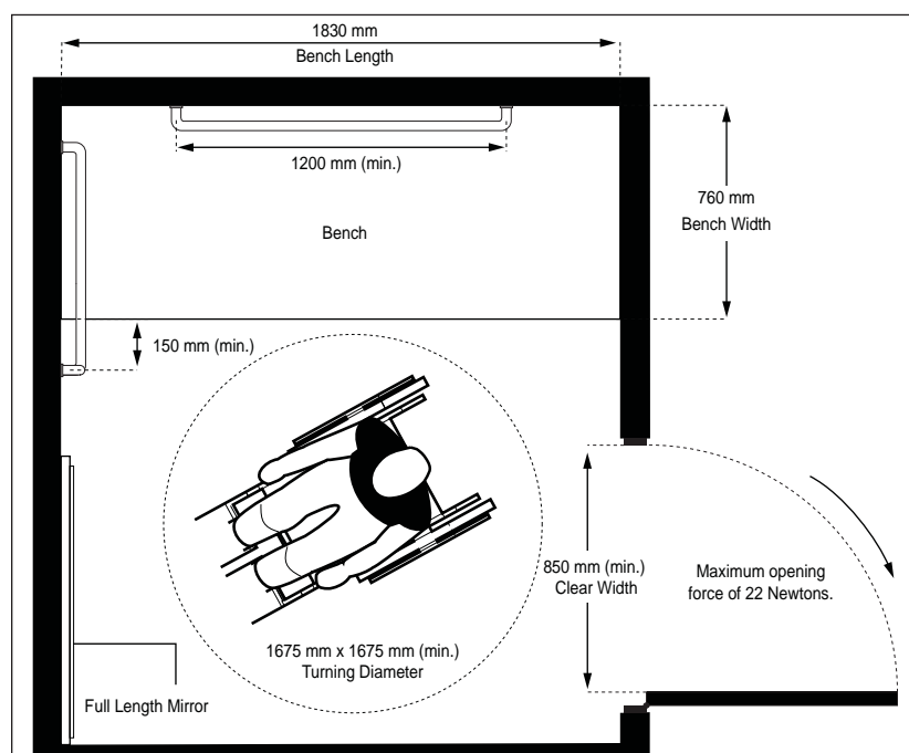
Figure 92a: Universal Change Room - Plan View
