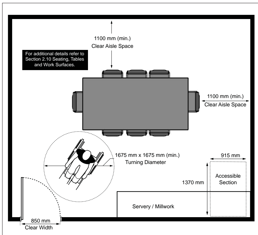
Figure 79: Meeting Room Design and Layout
