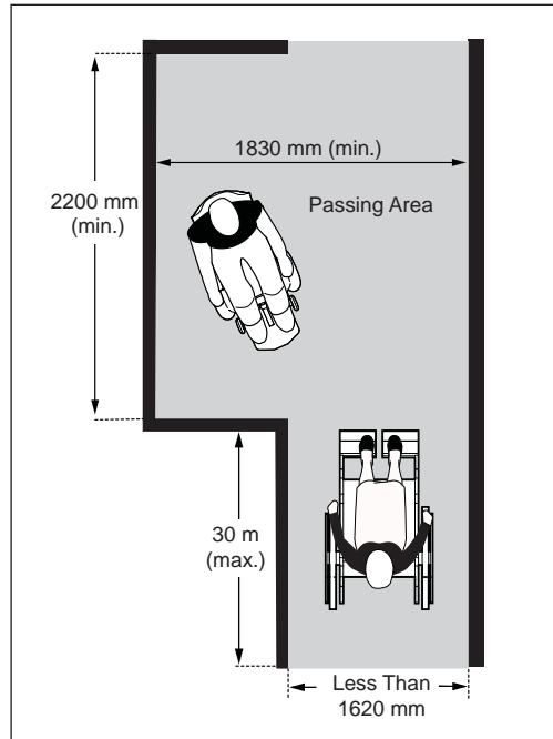
Figure 46b: Required Passing Area for Routes Greater than 30 metres
