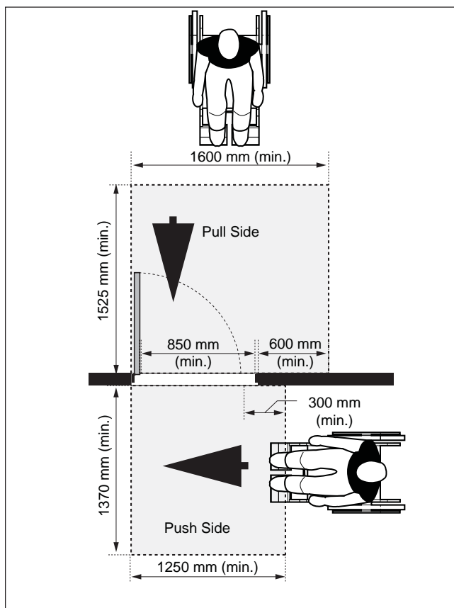
Figure 41a: Front and Side Approach at Side-Hinged Door - Plan View
