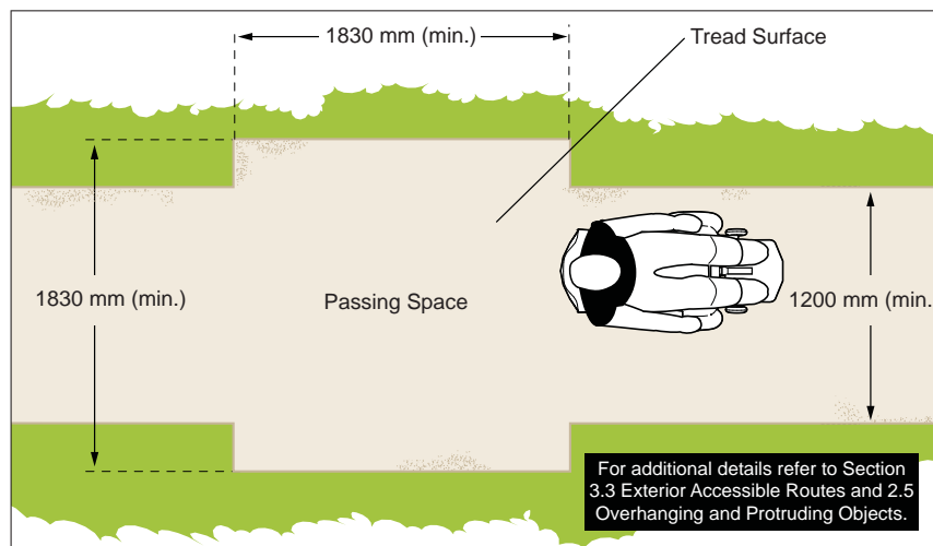
Figure 99: Tread Clear Width
