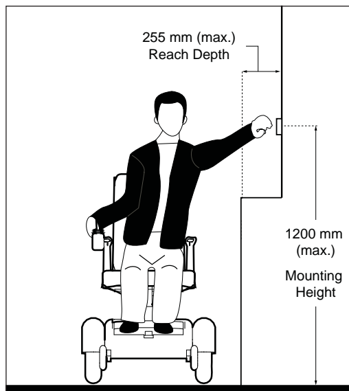
Figure 66a: Obstructed Side Approach and Reach: Depth 255 mm (Maximum)
