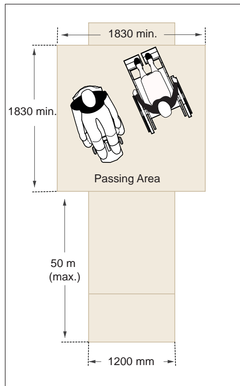
Figure 29b: Reduced Clear Width and Required Passing Area
