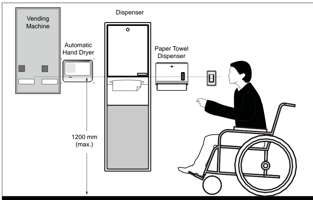
Figure 58: Typical Washroom Amenities
