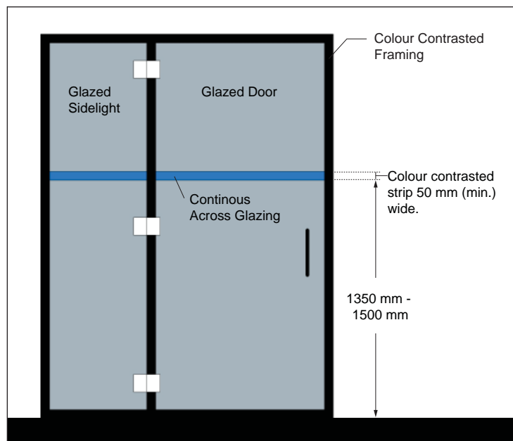
Figure 44: Glazed Doors - Elevation View
