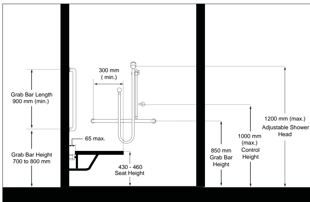
Figure 62: Grab Bars - Section View
