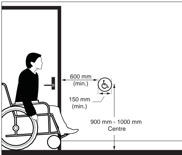
Figure 40a: Circular Push Button - Elevation View
