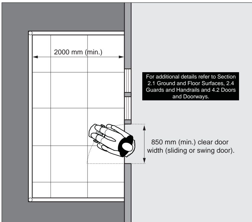
Figure 93: Balcony / Terrace - Plan View
