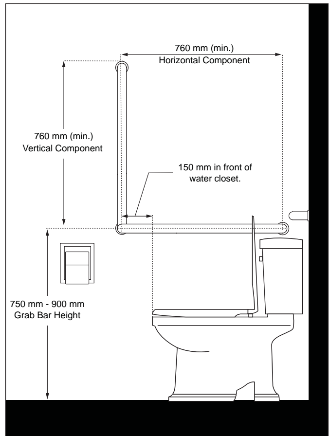
Figure 55: L-Shaped Grab Bar
