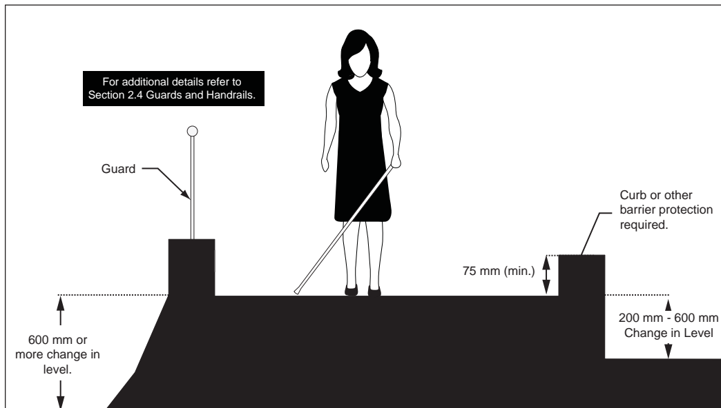
Figure 31: Changes in Level - Section View
