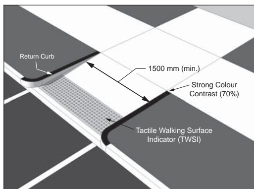
Figure 33a: Return Curb
