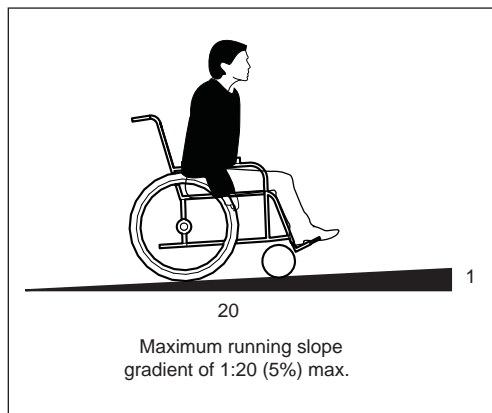
Figure 48: Running Slope
