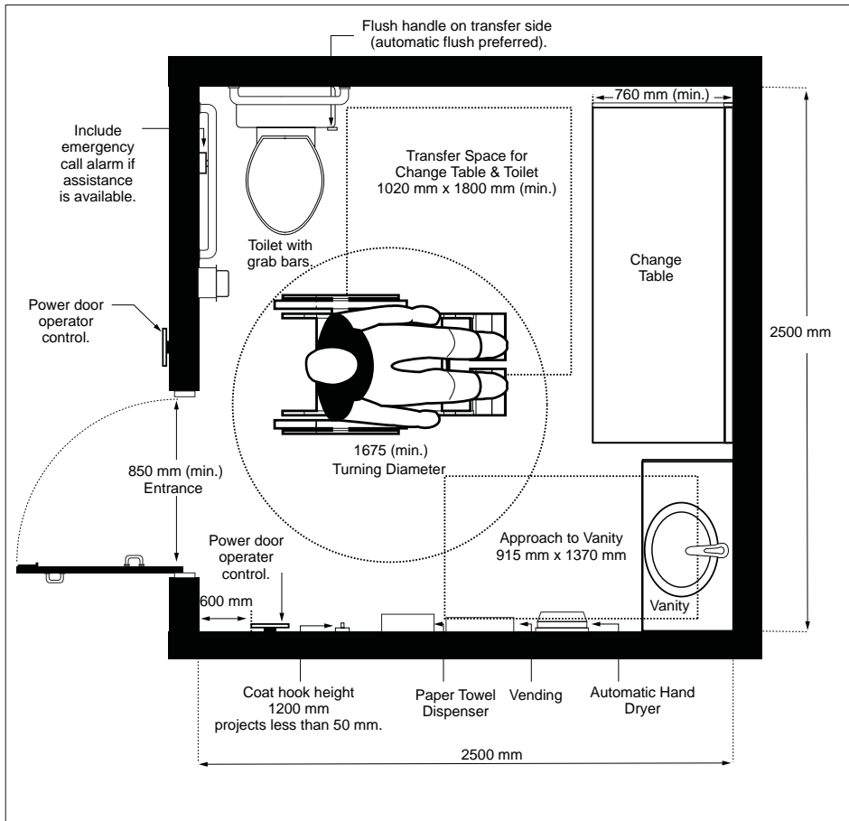
Figure 51: Universal Toilet Rooms
