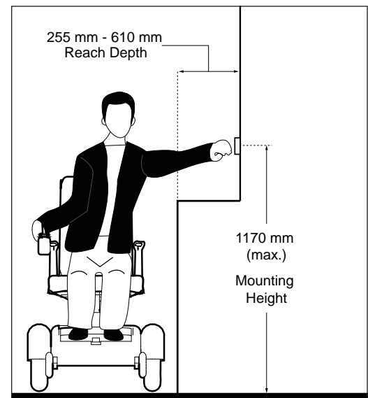
Figure 66b: Obstructed Side Approach and Reach: Depth 255 to 610 mm (Maximum)
