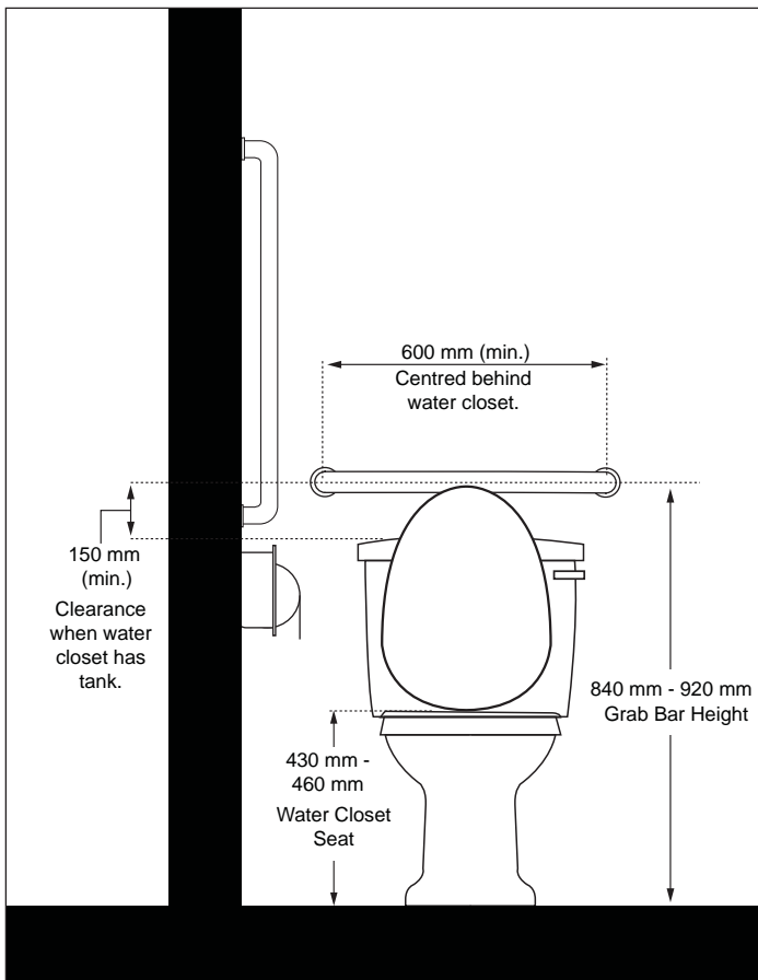
Figure 54: Horizontal Grab Bar
