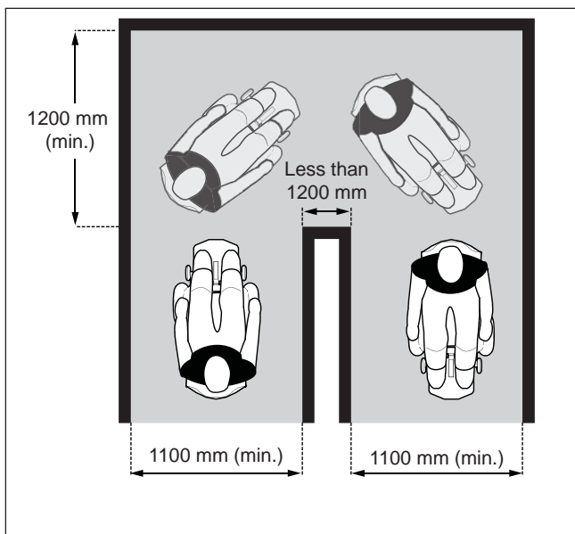
Figure 47a: 180 Degree Turn (Typical)
