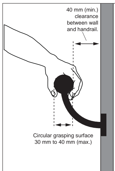
Figure 13a: Handrails on Wall - Section View
