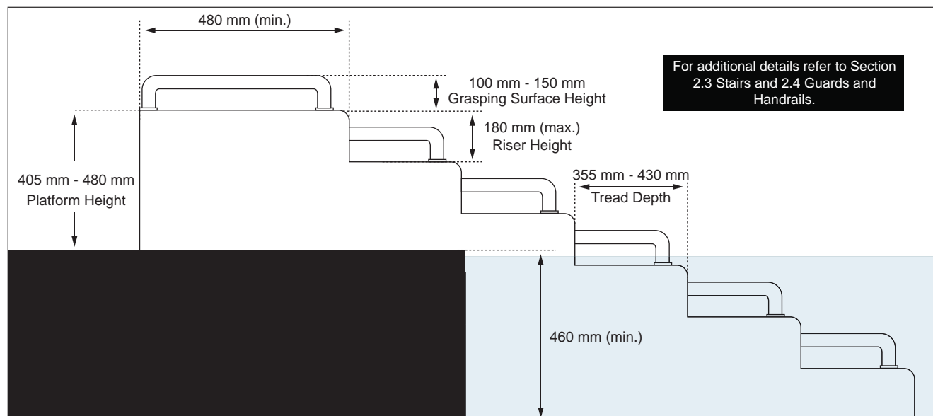
Figure 90: Transfer Stairs or Steps - Elevation View
