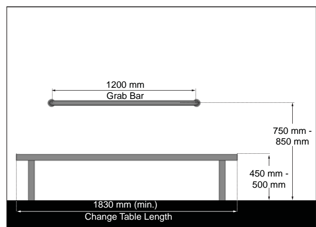
Figure 59b: Fixed Adult Change Table - Front View
