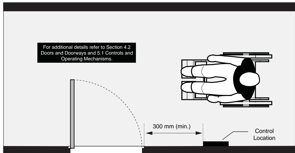
Figure 67: Proximity Card Reader Location - Plan View
