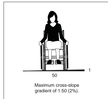
Figure 30b: Cross-Slope
