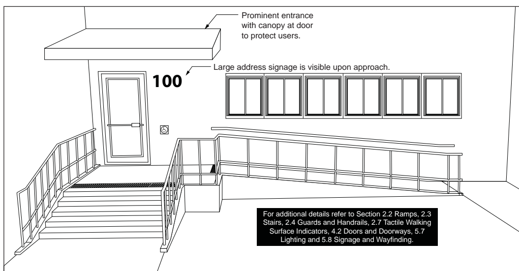
Figure 35: Main or Primary Entrance Features
