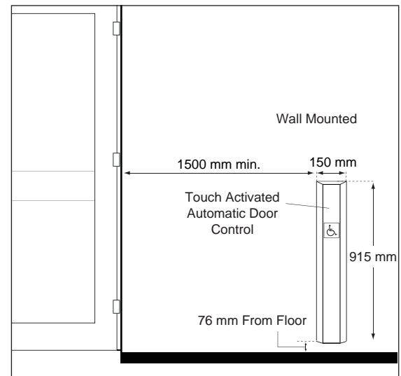
Figure 40b: Touch Activation Device - Elevation View
