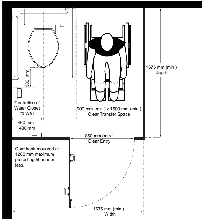
Figure 53: Water Closets
