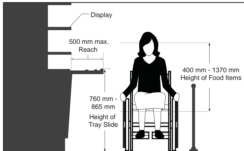
Figure 80a: Food Displays and Tray Slides - Section View
