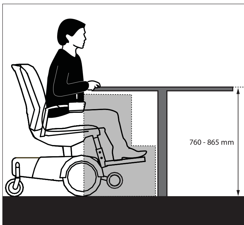
Figure 23a: Table and Work Surface - Elevation View
