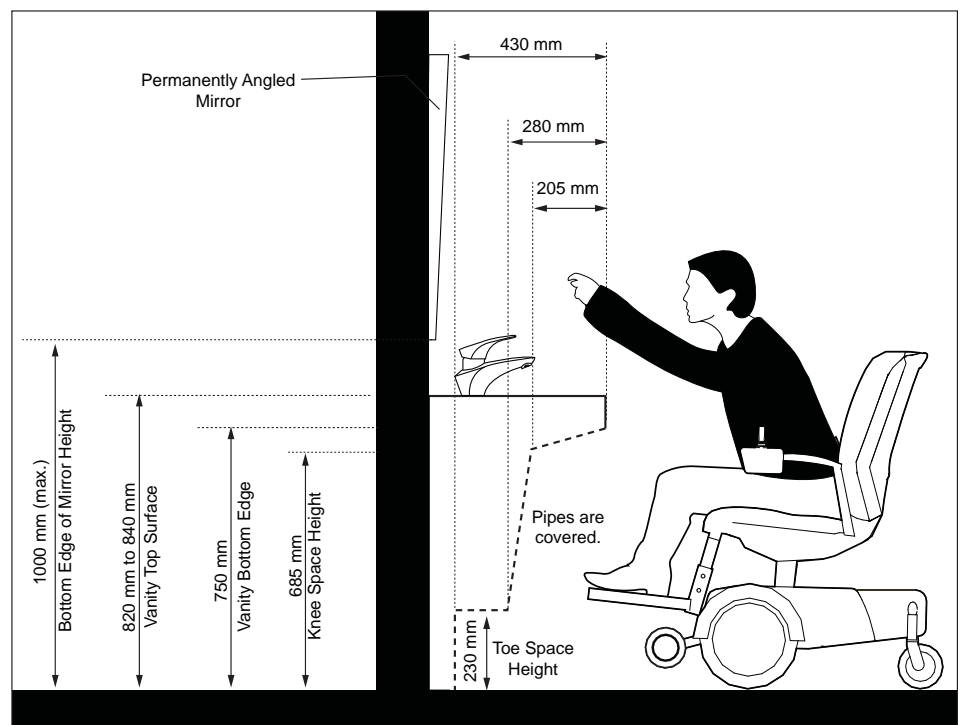
Figure 57b: Lavatories - Section View
