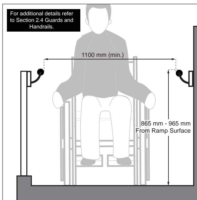
Figure 8: Handrail Design and Features - Section View
