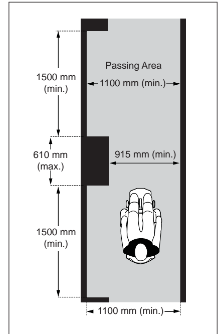
Figure 46c: Permitted Reduced Clear Width
