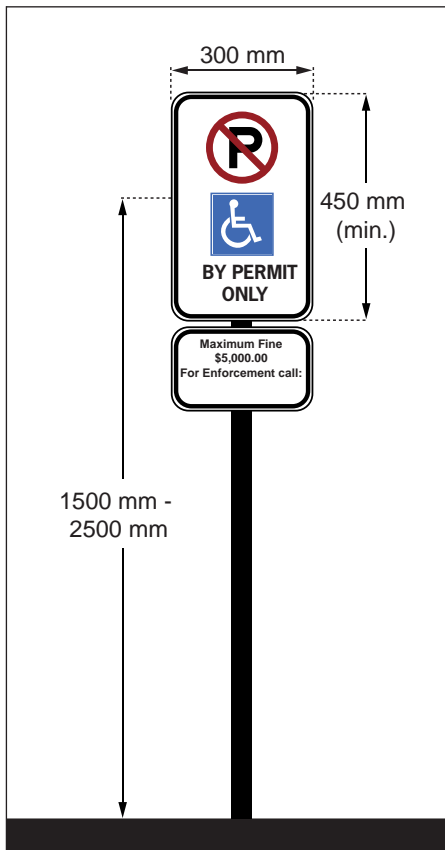
Figure 25: Accessible Parking Vertical Signage
