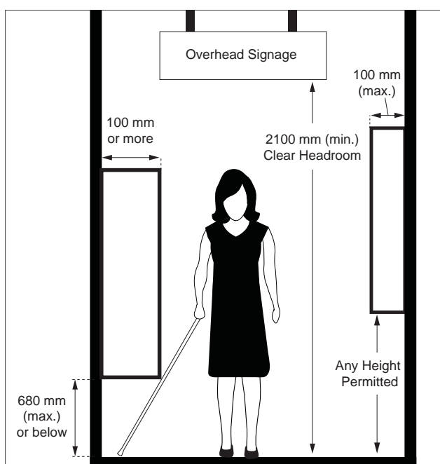
Figure 15: Protruding Objects
