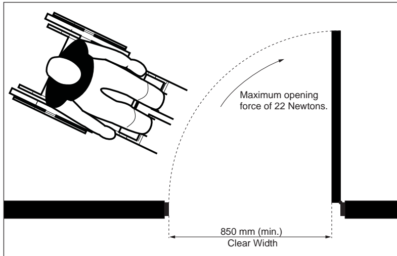
Figure 37: Clear Width of Doors
