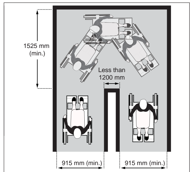
Figure 47b: 180 Degree Turn - Exception
