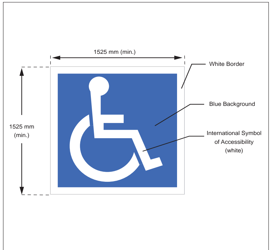
Figure 26: Accessible Parking Pavement Markings
