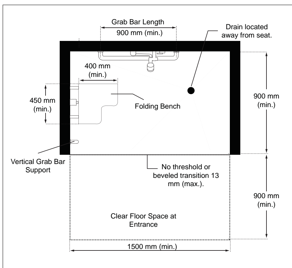
Figure 61: Shower Design and Layout - Plan View
