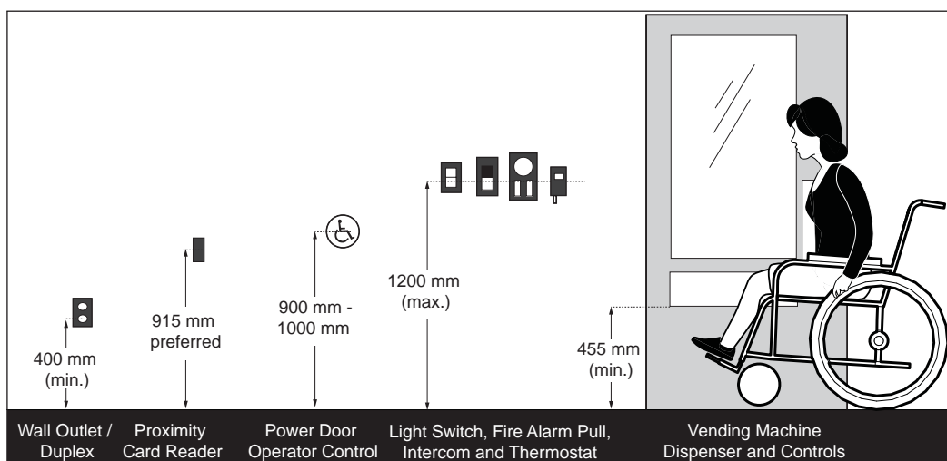
Figure 64: Control Mounting Heights - Elevation View
