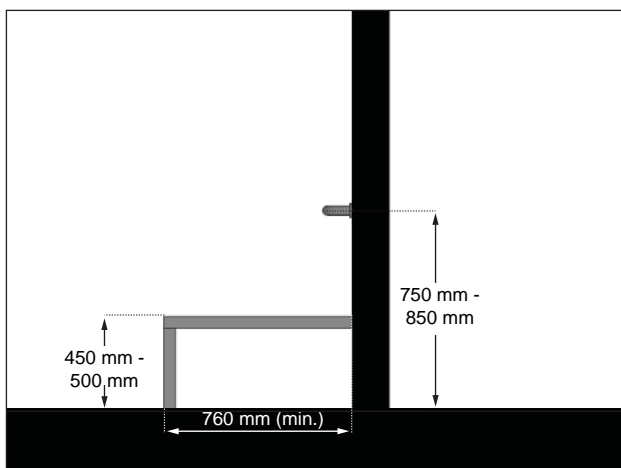
Figure 59a: Fixed Adult Change Table - Section View
