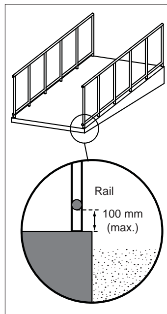
Figure 4c: Rail Protection
