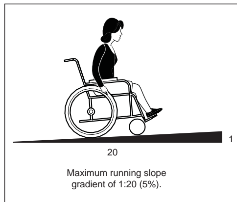
Figure 30a: Running Slope
