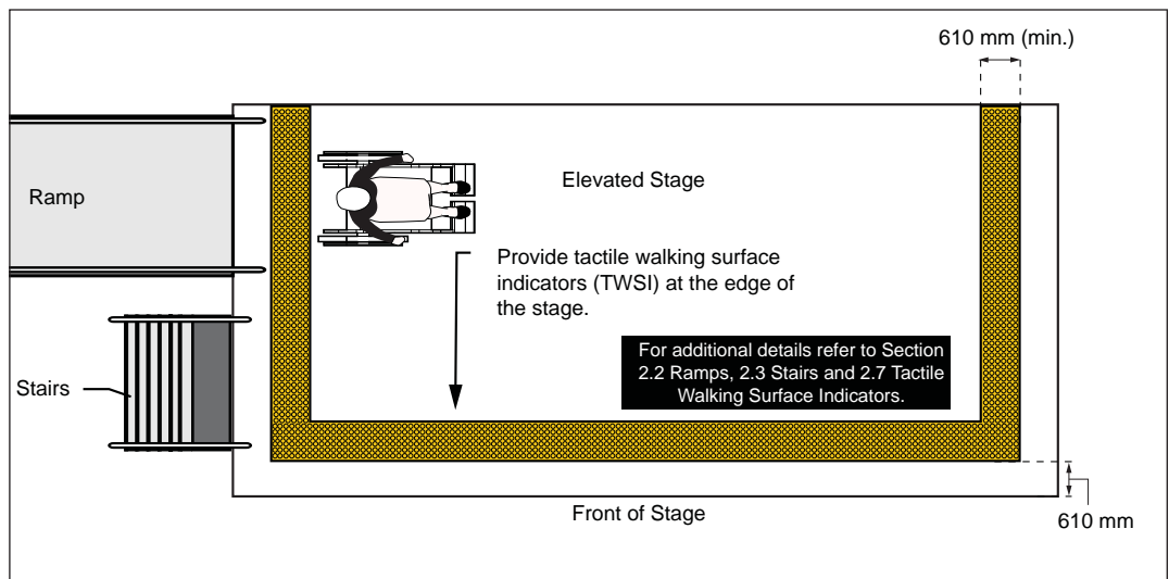
Figure 96: Elevated Platform or Stage - Plan View
