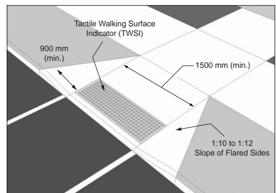
Figure 33b: Flared Sides
