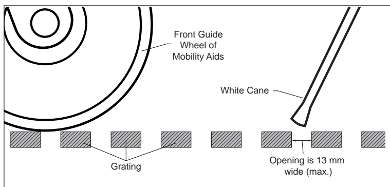
Figure 2b: Gratings - Section View
