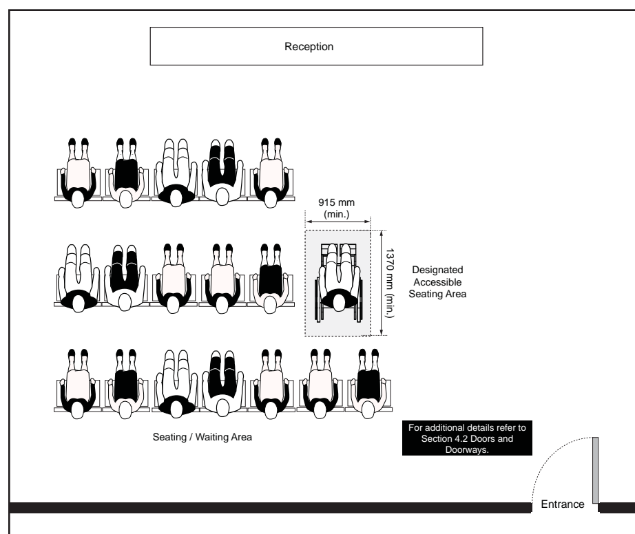
Figure 36: Lobby and Waiting Area - Plan View
