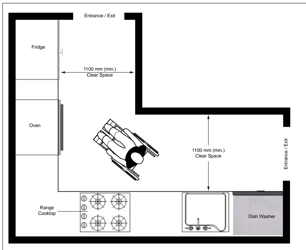
Figure 83: L-Shaped Kitchen - Plan View
