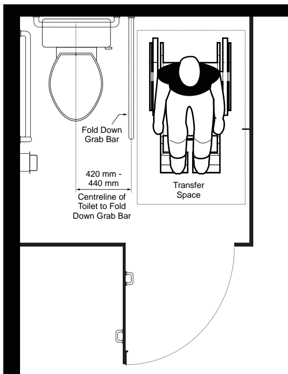
Figure 56a: Fold Down Grab Bars - Plan View
