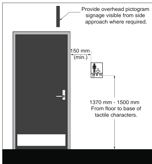
Figure 70: Mounting Height and Provisions of Permanent Signage - Elevation View
