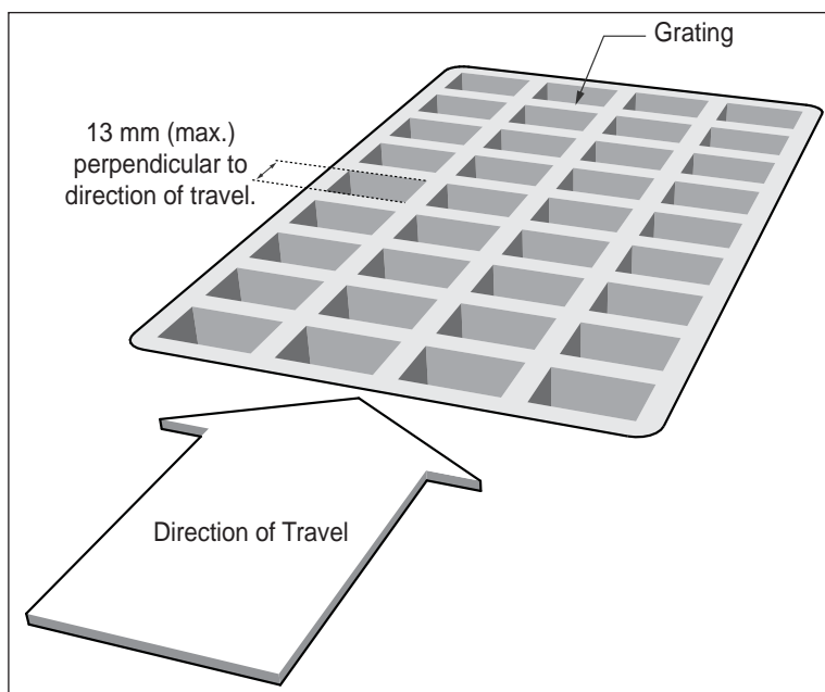
Figure 2a: Grating Opening
