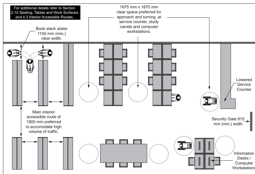
Figure 85: Library Design and Layout - Plan View
