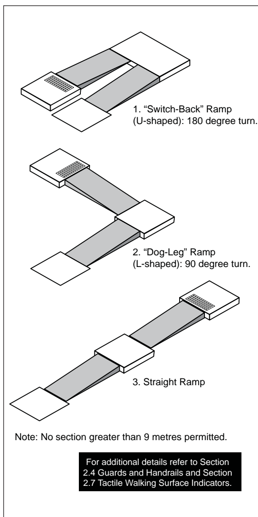
Figure 5: Typical Ramp Configurations
