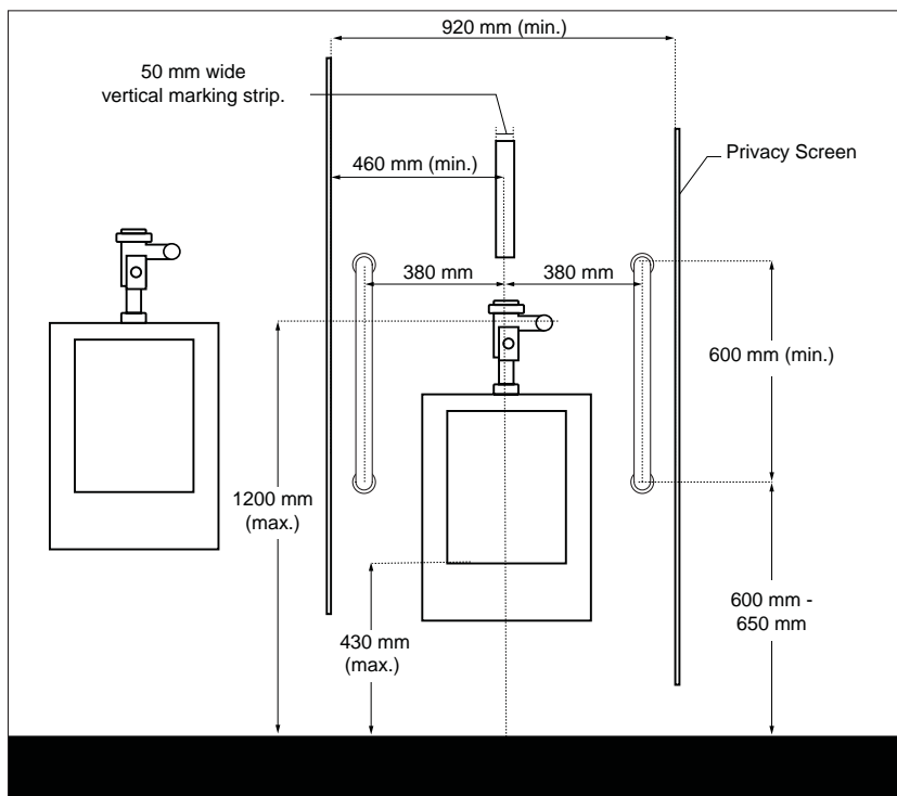
Figure 60: Urinals - Elevation View
