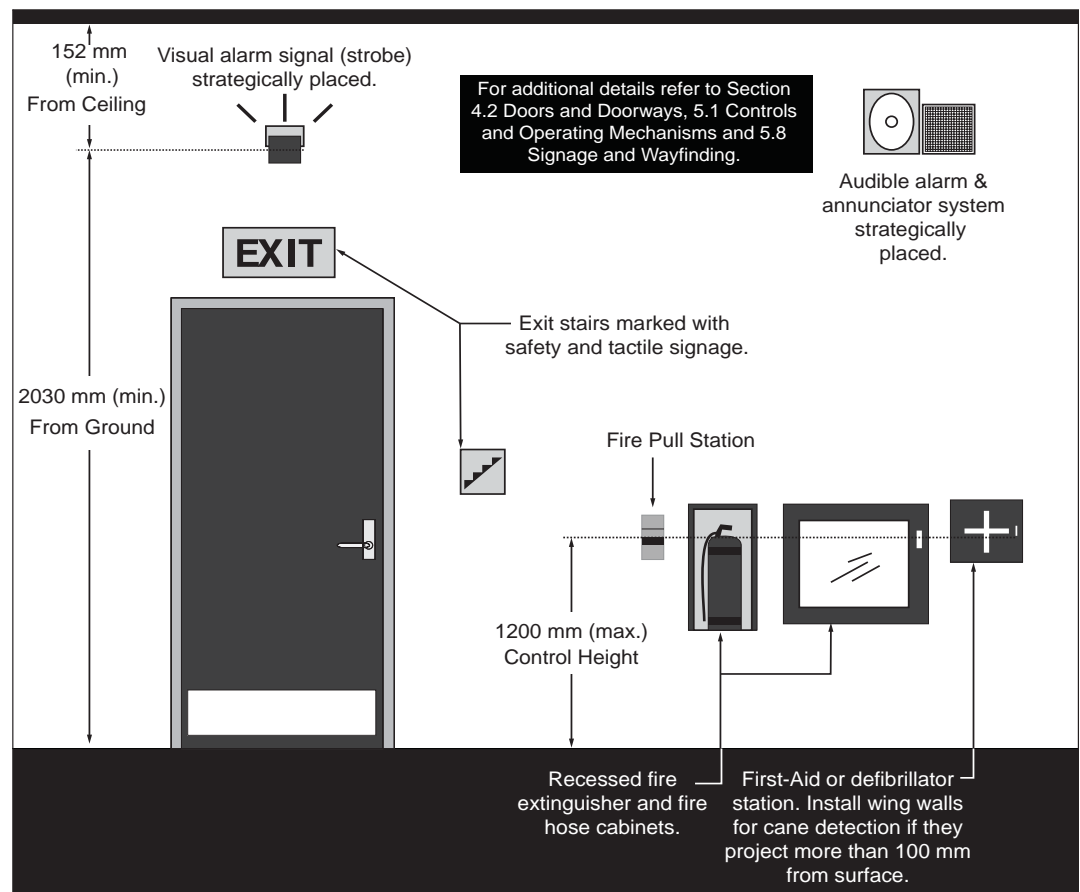
Figure 68: Fire Safety and Evacuation Features - Elevation View
