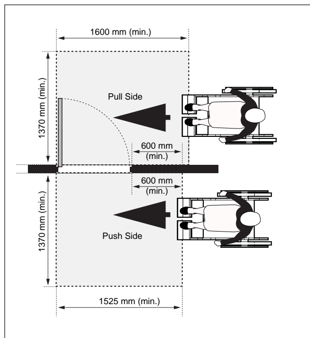
Figure 41d: Latch Side Approach at Side-Hinged Door - Plan View
