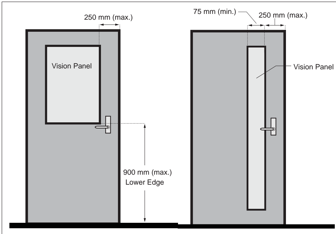
Figure 45: Vision Panels - Elevation View
