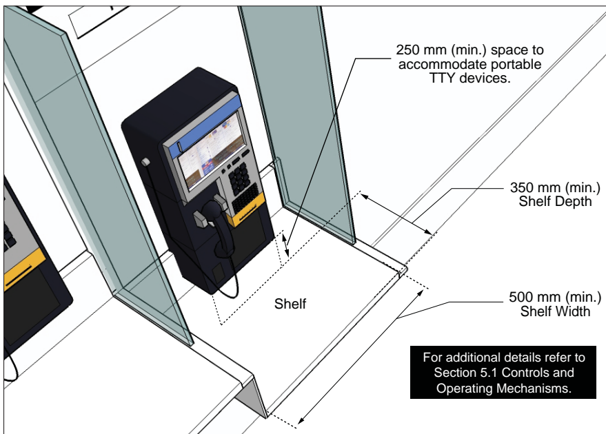
Figure 21: Shelf Dimensions for Public Telephones
