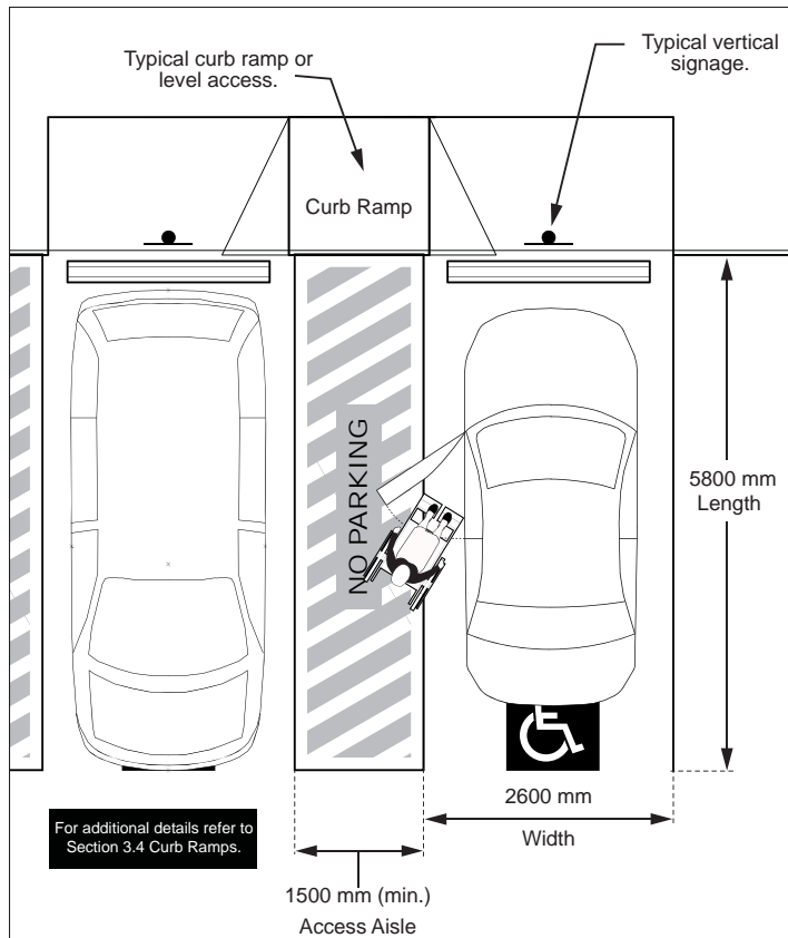
Figure 24: Accessible Parking Space Dimensions - Plan View
