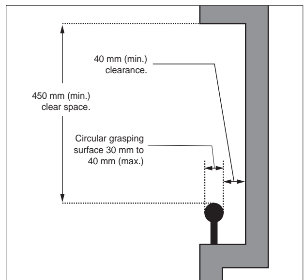
Figure 13b: Handrails in Recessed Area - Section View
