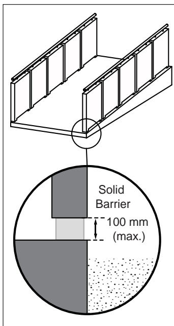
Figure 4b: Solid Barrier Protection
