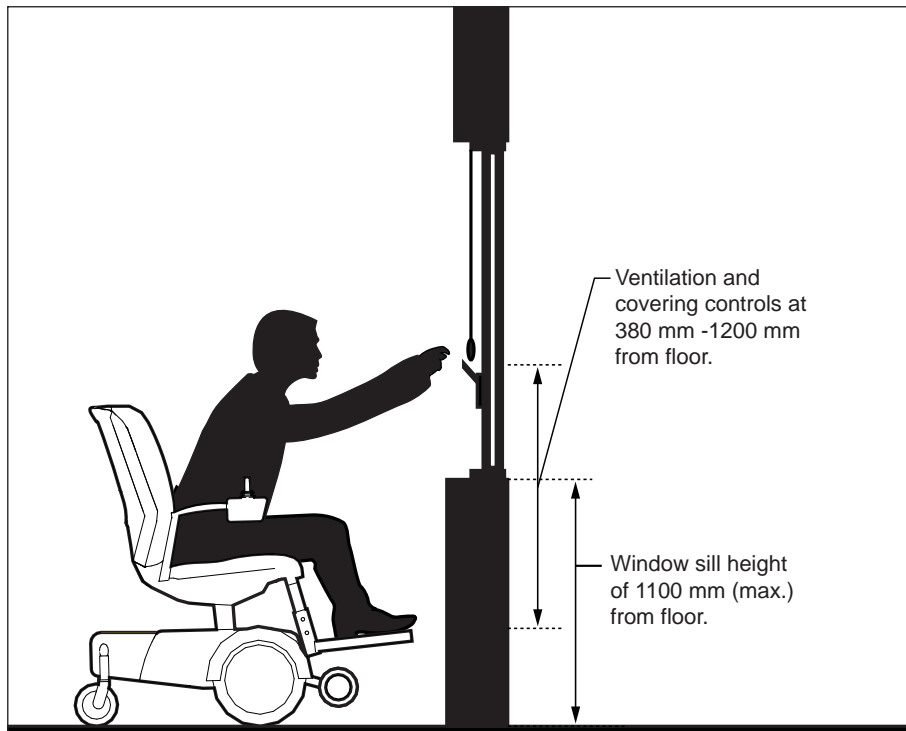
Figure 75: Window Design Features - Elevation View
