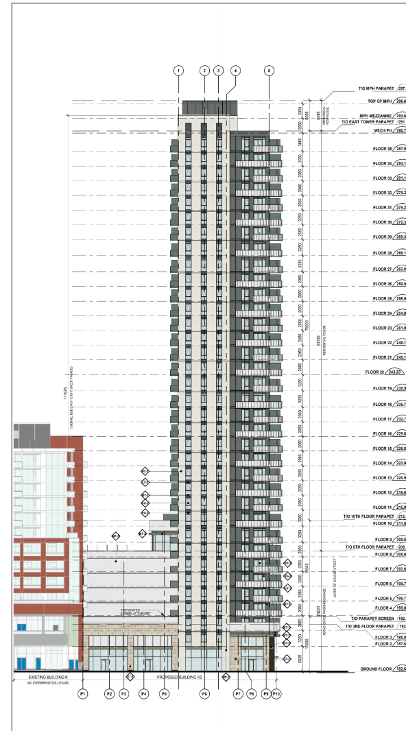
1 SOUTH ELEVATION A402.S
