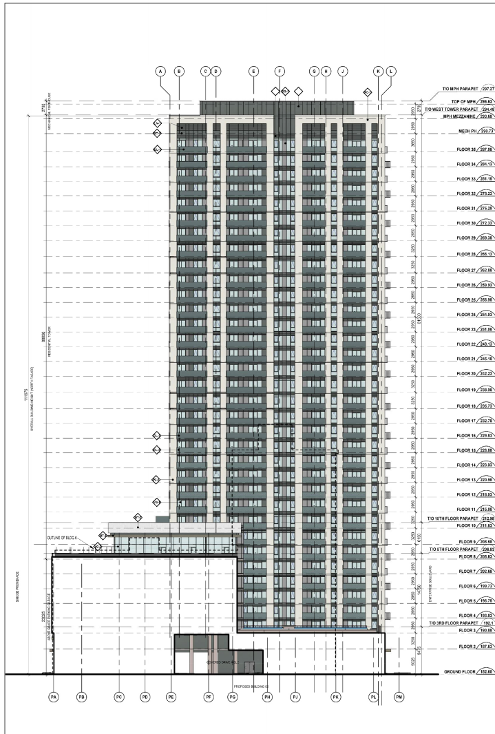
2 WEST ELEVATION A402.S
