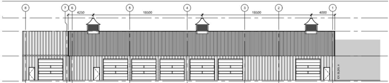
PAVED STEEL BLDG - EAST ELEVATION
