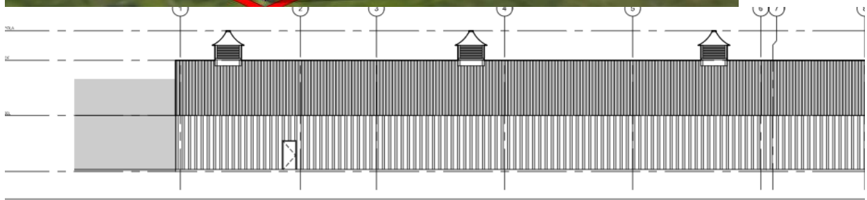
PAVED STEEL BLDG - EAST ELEVATION
