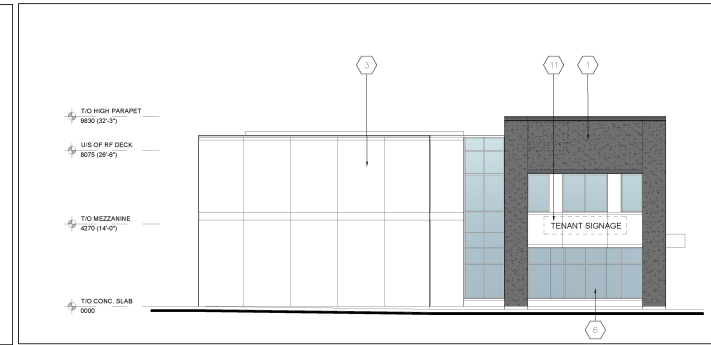
2 SOUTH ELEVATION A-3.0 1:200
