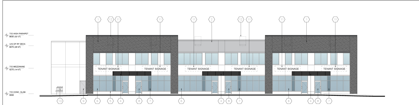
3 EAST ELEVATION A-3.0 1:200
