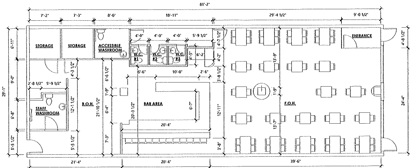
1 FLOOR PLAN 1" = 10'-0"
