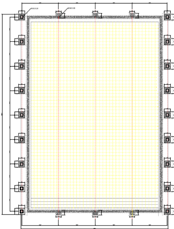
PROPOSED RINK FOUNDATION PLAN
