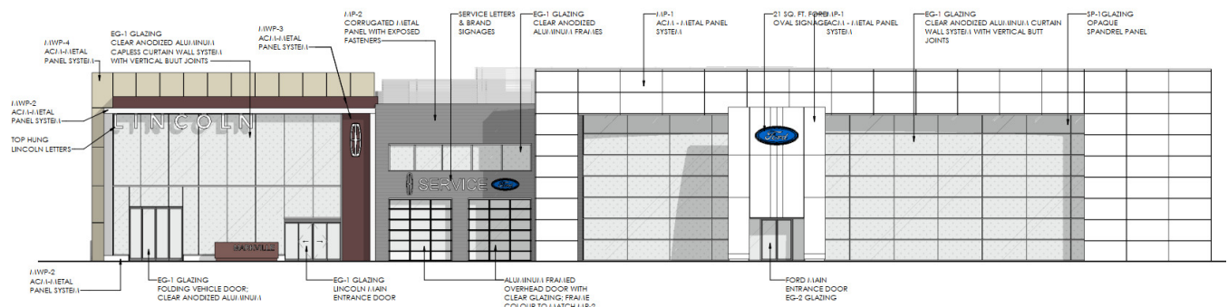
2 SOUTH ELEVATION A3.02 1 : 150
